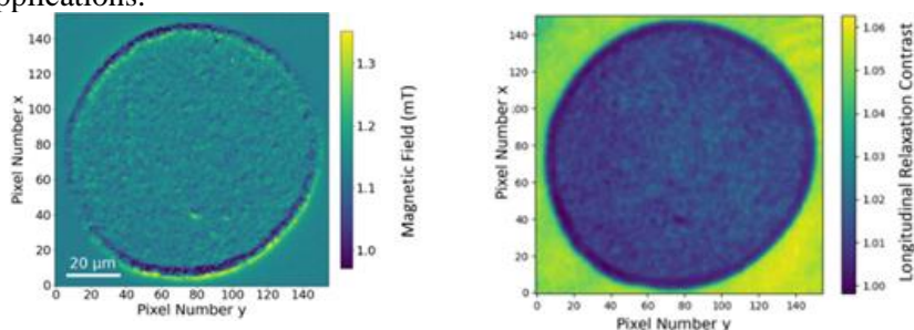
Figure 1: Left: Magnetic field component generated by magnetic nanoparticles reconstructed from the measured Zeeman splitting of the NV-center spin states. Right: Longitudinal relaxation contrast image of NV centers induced by MNP GHz noise.
