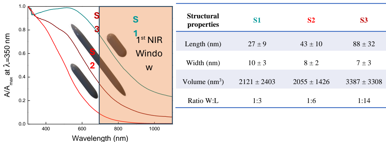
Figure 1: left) Normalized optical absorption spectra of Bi 2 S 3 Nanorods with various morphologies. Right) table of nanorod dimensions for each sample. References
