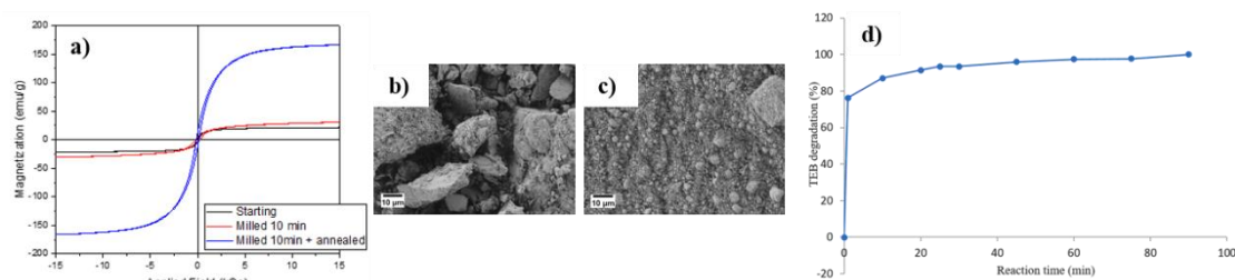
Figure 1: (a) Room temperature hysteresis loops measured by vibrating sample magnetometry (VSM) for the precursor powder and that after milling for 10 min before and after annealing. Scanning electron microscopy (SEM) images of (b) the starting powder and (c) the powder milled for 10 min. (d) Percentage degradation of tebuconazole during a CWPO process using the NPs as catalyst.
