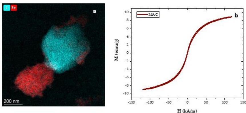
Figure 1. HRTEM image of the MAC sample (a). Magnetic characterization (b).
