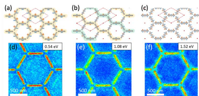
Figure 1. Plasmonic modes measured in the lattice at three different energies. (a), (b) and (c) show schematic representations of the charge distributions associated with a bright mode and two examples of extended and local dark modes, respectively. Panels (d), (e) and (f) present the EELS mapping for each of the modes depicted in the upper panels.
