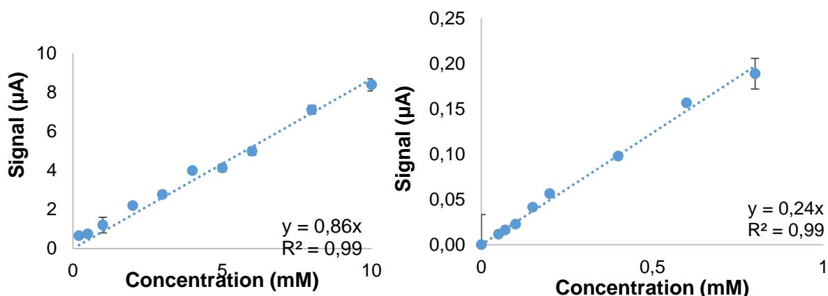
Figure.1 Linear range with microelectrode LIG/Ni/Cu in neutral media.
