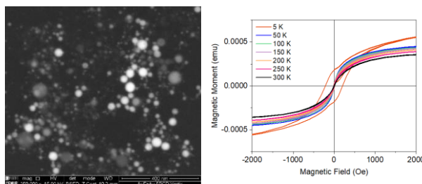
Figure 1: Nanoparticles synthesized via laser ablation of an Iron and Gold target (left); Nanoparticle's magnetization versus magnetic field measurements at different temperatures (right).
